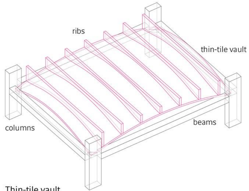
Thin-tile vault
